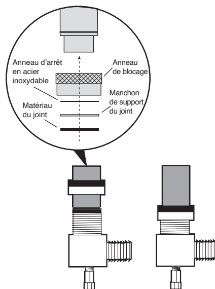
Figure 4 : Raccords pivotants
