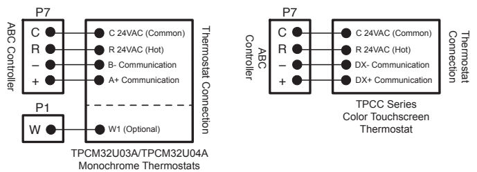
Figure 22: Thermostat Wiring (Communicating Style Signals)
