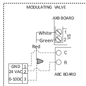
Figure 1c: Modulating Water Valve Connection Option Typical 0-10VDC modulating water valve.
