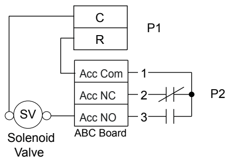
Figure 1a: Open Loop Solenoid Valve Connection Option Typical quick operating external 24V water solenoid valve (type PPV100 or BPV100) wiring.
