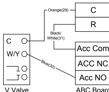
Figure 1b: Open Loop Solenoid Valve Connection Option Typical slow operating external 24V water solenoid valve (type V100FPT) wiring.
