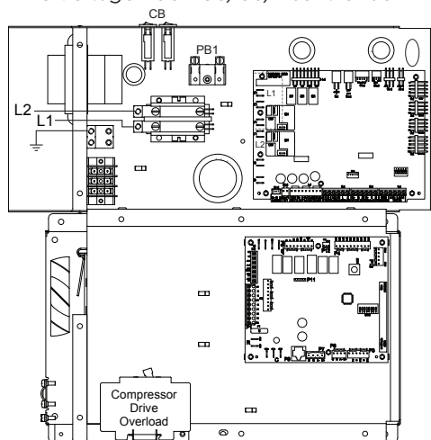
Figure 13c: Line Voltage 208-230/60/1 control box
