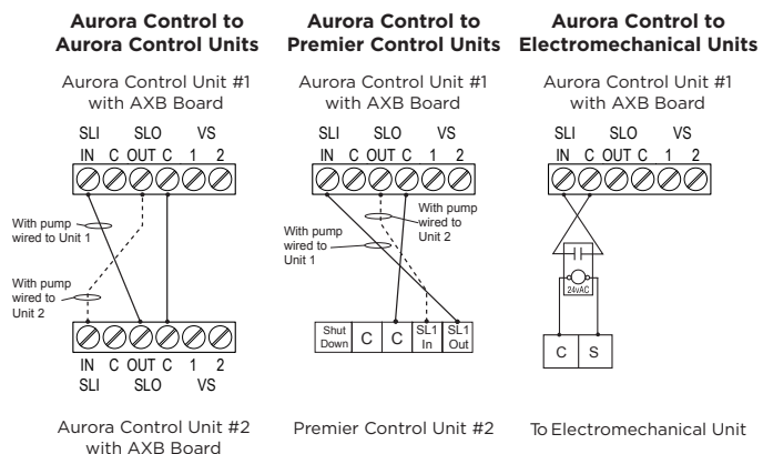
Figure 8: Primary/Secondary Hook-up
