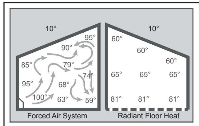
Figure 5: Temperature Comparison
