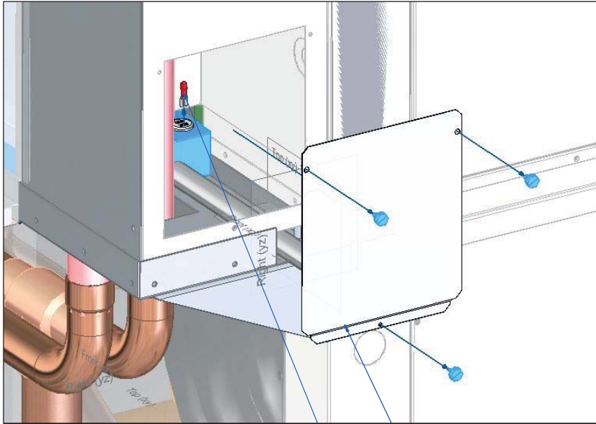
ECONOMIZER ACCESS PANEL ECONOMIZER OVERFLOW DRAIN SWITCH TERMINAL
